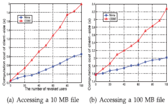
Fig. 3.2. Comparison on computation cost for file access between Mona and ODBE.
