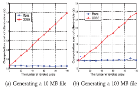
Fig. 3.1. Comparison on computation cost for file generation between Mona and ODBE.
